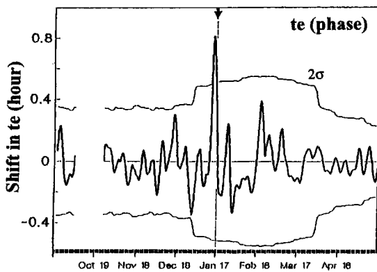
Fig. 2. Change in terminator time (here t_e , phase) for a longer period ( \pm 4 months around the quake). The thick line is the average shift from the mean over \pm 1 day at each day. A significant change (exceeding 2\sigma line) is seen only before the quake.
