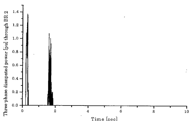
Fig. 23. Dissipated power response for BR 2
