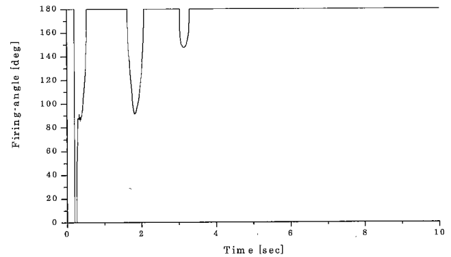
Fig. 20. Firing-angle response for BR 1
