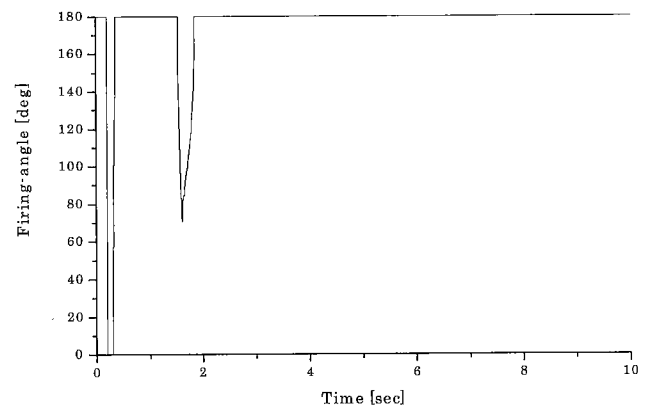
Fig. 21. Firing-angle response for BR 2
