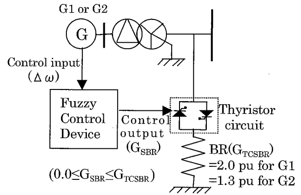
Fig. 2. BR with thyristor switching circuit
