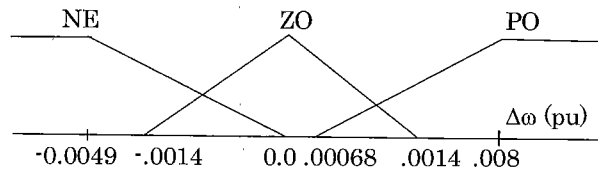
Fig. 8. Membership function of \Delta\omega by trial and error
