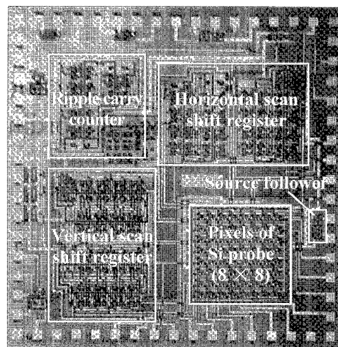
Fig. 4. Photograph of a fabricated chip.
