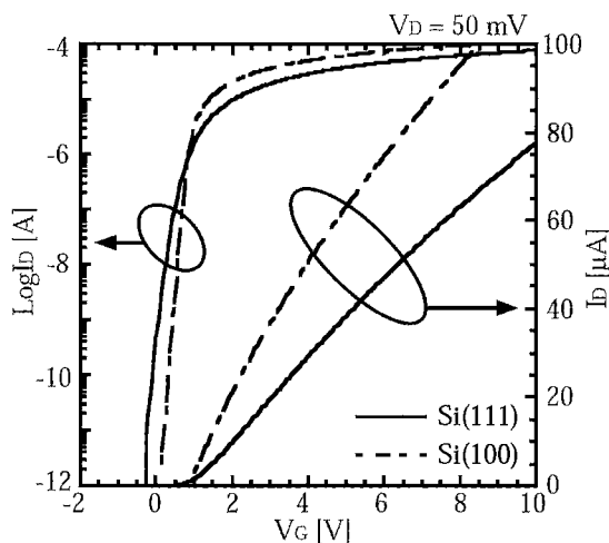
Fig. 5. I_D - V_G characteristics of n-MOSFET on Si (111) and Si (100).
